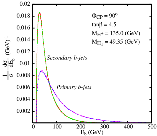
Fig. 4. The energy distributions of the two “primary” and two “secondary” b -jets in the signal (as defined in the text), as obtained for the representative parameter choices shown inside the figure
