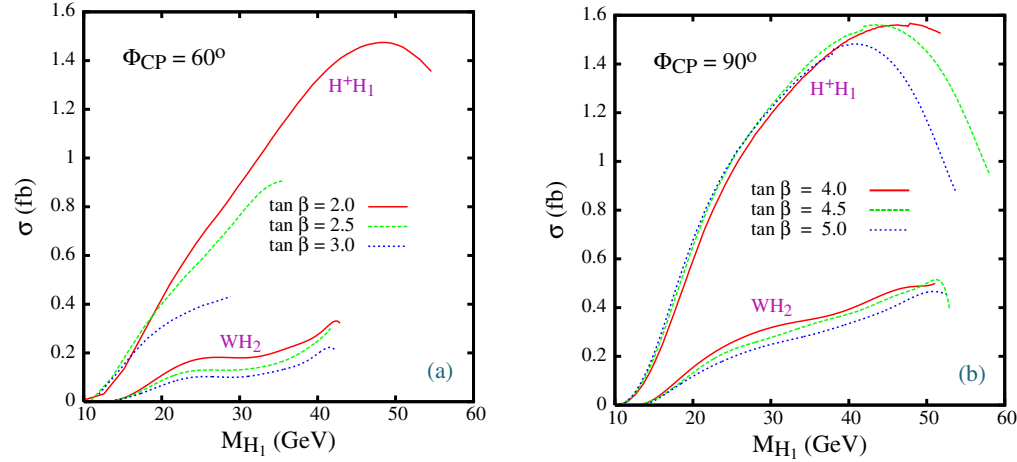
Fig. 2. A comparison between the production rates of the two processes q\bar{q}' \rightarrow H_2 W^\pm \rightarrow H_1 H_1 W^\pm \rightarrow b\bar{b}b\bar{b}l\nu and q\bar{q}' \rightarrow H_1 H^\pm \rightarrow H_1 H_1 W^\pm \rightarrow b\bar{b}b\bar{b}l\nu , for \Phi_{CP} = 60^\circ (a) and \Phi_{CP} = 90^\circ (b), for the three choices of \tan\beta shown in the figure
