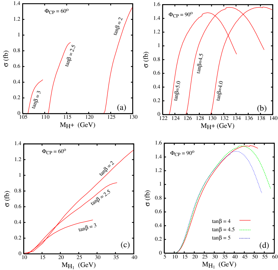
Fig. 1. Variation of the signal cross-section with M_{H^\pm} [a, b] and M_{H_1} [c, d] for the two values of CP -violating phases \Phi_{CP} = 60^\circ [a, c] and \Phi_{CP} = 90^\circ [b, d]. The choices of \tan\beta for each CP -violating phase are shown in the figure
