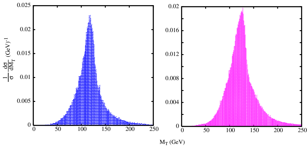
Fig. 5. The transverse mass distribution (as defined in the text) for the signal, for M_{H^\pm} = 129.55 GeV (left panel) and M_{H^\pm} = 135 GeV (right panel), \tan\beta = 4.5 and \Phi_{CP} = 90^\circ
