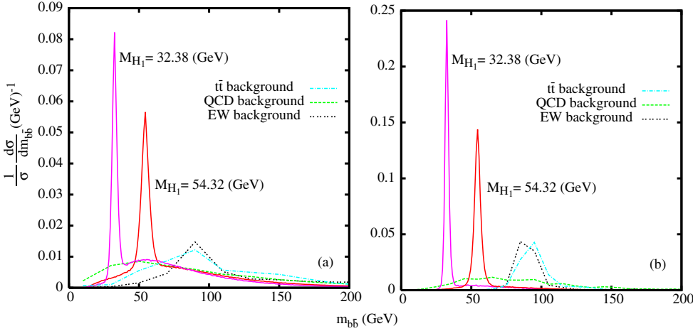
Fig. 3. The “average” a and “best reconstructed” b m_{b\bar{b}} distributions (as described in the text) for the signal (with M_{H_1} = 32.38 and 54.32 GeV, corresponding to M_{H^\pm} = 129.55 and 136.97 GeV, respectively, for \tan\beta = 4.5 and \Phi_{CP} = 90^\circ ). The corresponding SM model background distributions are also shown
